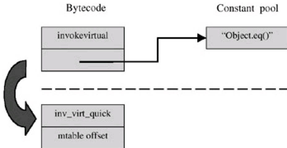
Figure 13.5: Optimizing invokevirtual by rewriting bytecode.
